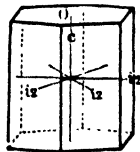
[11 \bar{2} 0]
